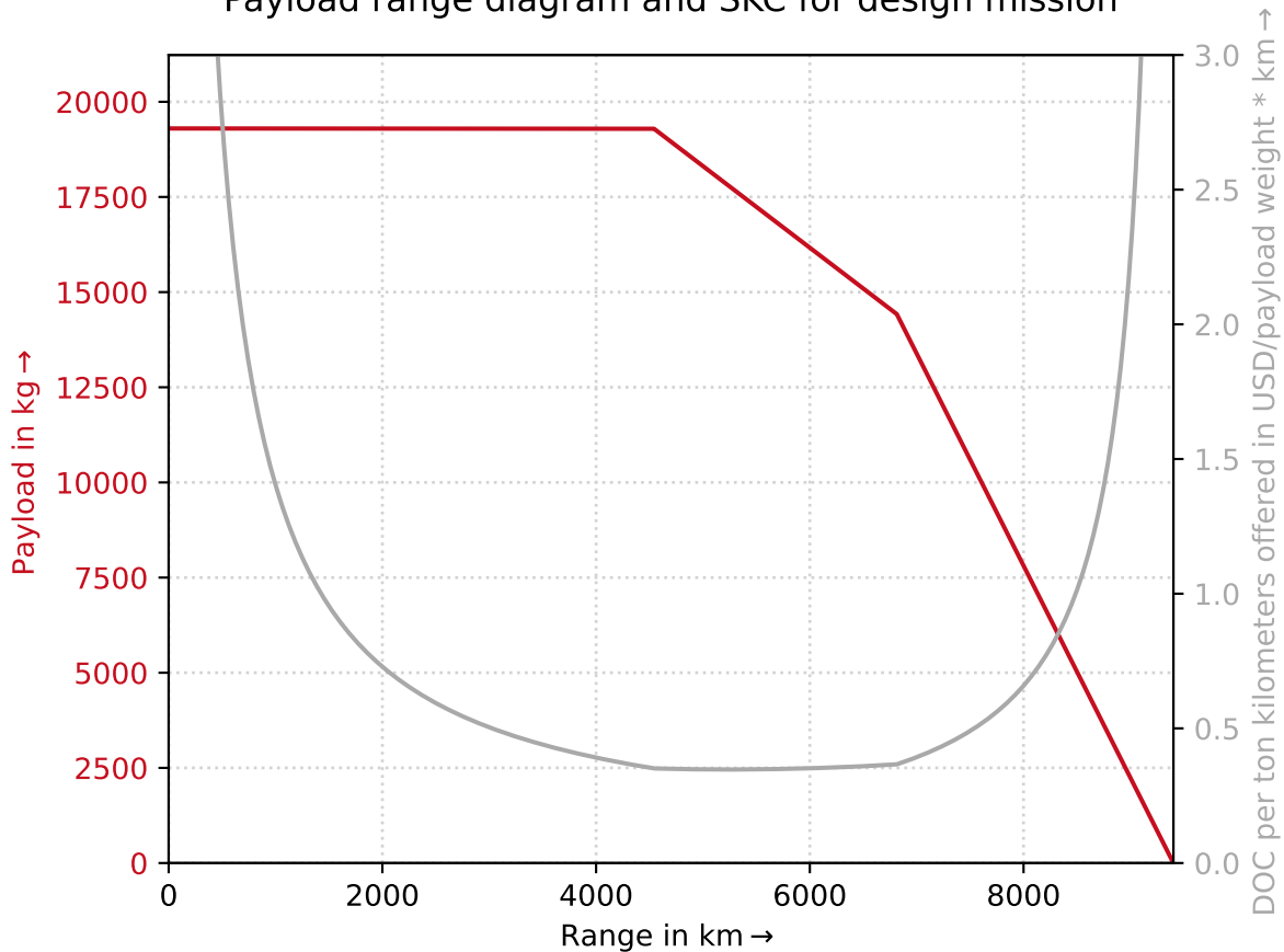
Payload range diagram and SKC for design mission
